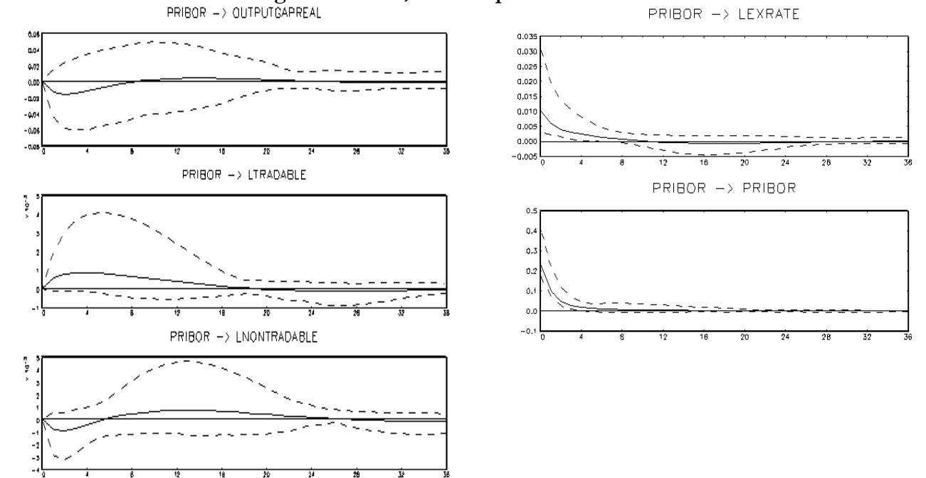
Figure 9: SVAR, sectoral prices
